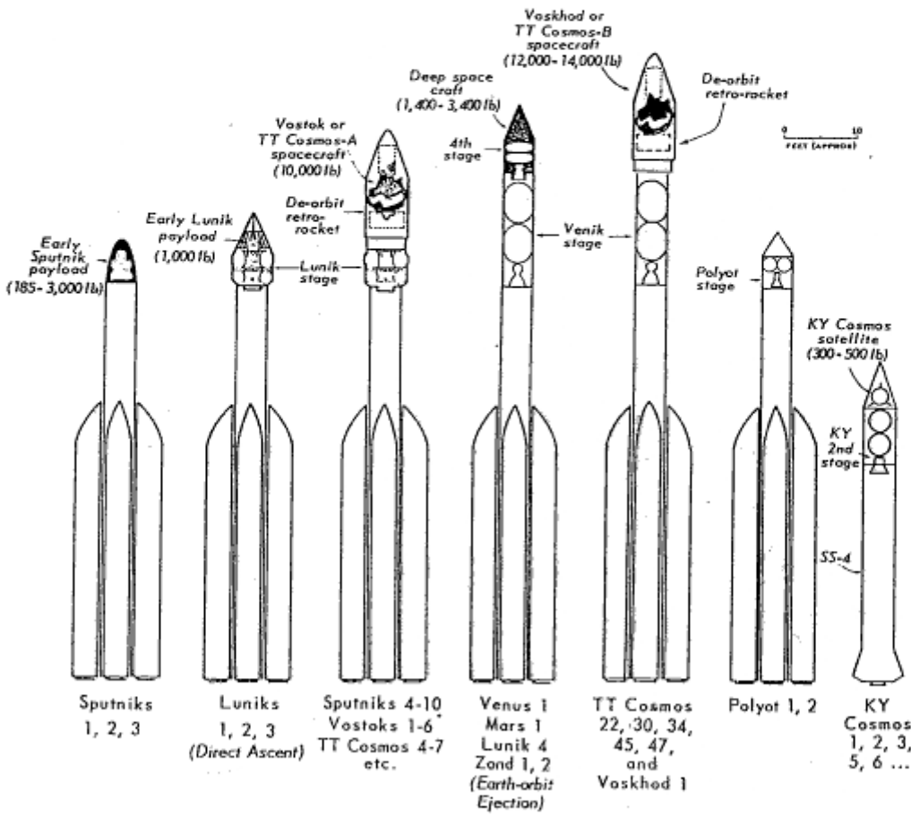
FAMILY OF SOVIET SPACE VEHICLES USED, 1957 - 1964
